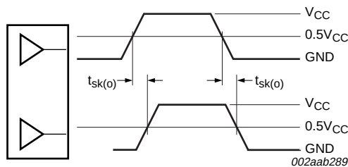
Fig 7. Pulse skew time ( t_{sk(p)} ) test reference
